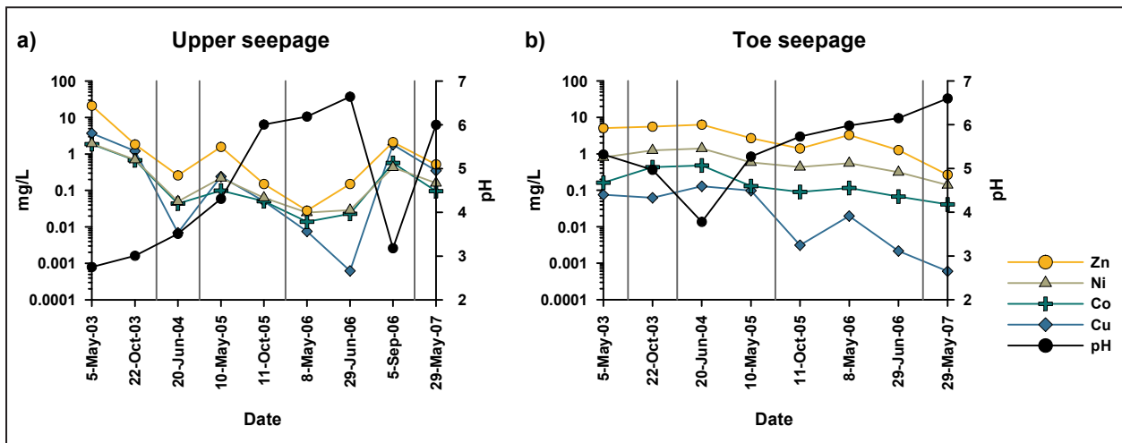
Figure 3. Diagram showing an example of the effect of local hydrological conditions and structural changes in the tailings impoundment seen in the metal concentrations (mg/L) and pH in the Luikonlahti tailings seepage waters between May 2003 and May 2007. a) 'Upper seepage' from the upper section of the tailings dam and b) 'toe seepage' from the toe of the dam. (Modified after Heikkinen et al. 2009).
