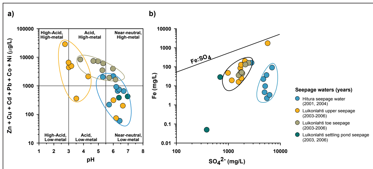
Figure 2. a) Variation in the seepage water quality from neutral to acid mine drainage in the low-sulphide Hitura tailings and the high-sulphide Luikonlahti tailings presented with a Ficklin diagram (Plumlee et al. 1999) showing the sum of dissolved heavy metals ( \mu\text{g/L} ) plotted against pH; b) Diagram of Fe versus \text{SO}_4^{2-} (mg/L) in the Hitura and Luikonlahti seepages. The diagonal black line indicates the Fe: \text{SO}_4 ratio produced by pyrrhotite weathering, which is typically one of the primary sources of Fe and \text{SO}_4 in tailings effluents.
